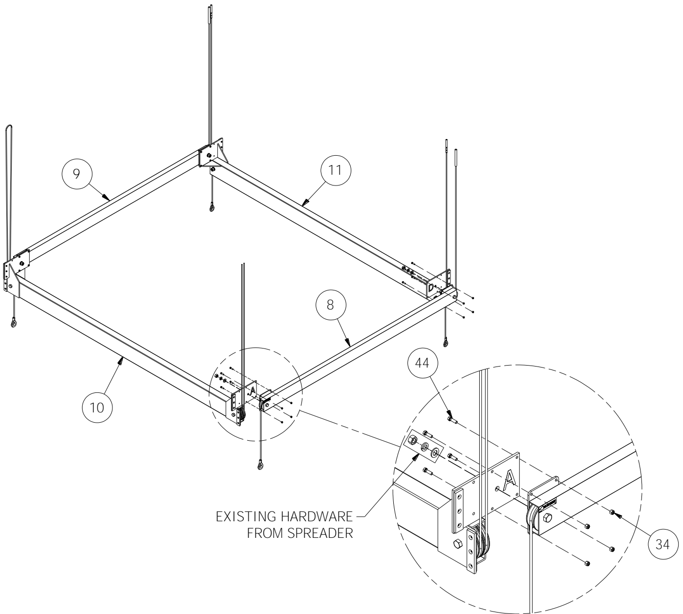
Platform Assembly – Top View
