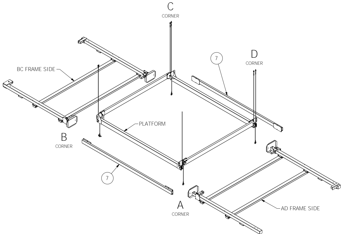
Layout of Assemblies to Assemble Frame
