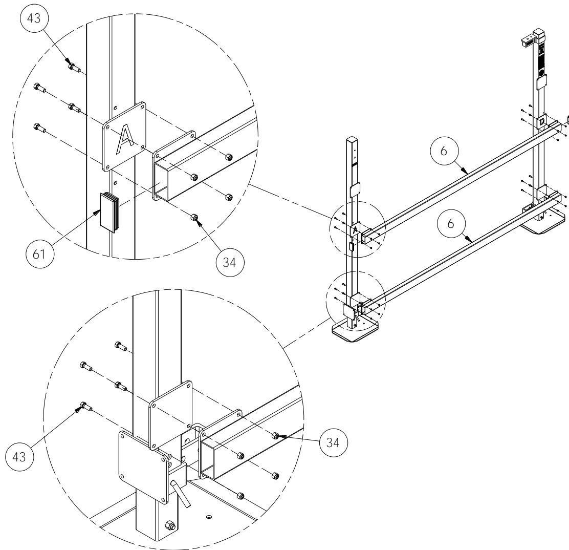
Frame Side Assembly
