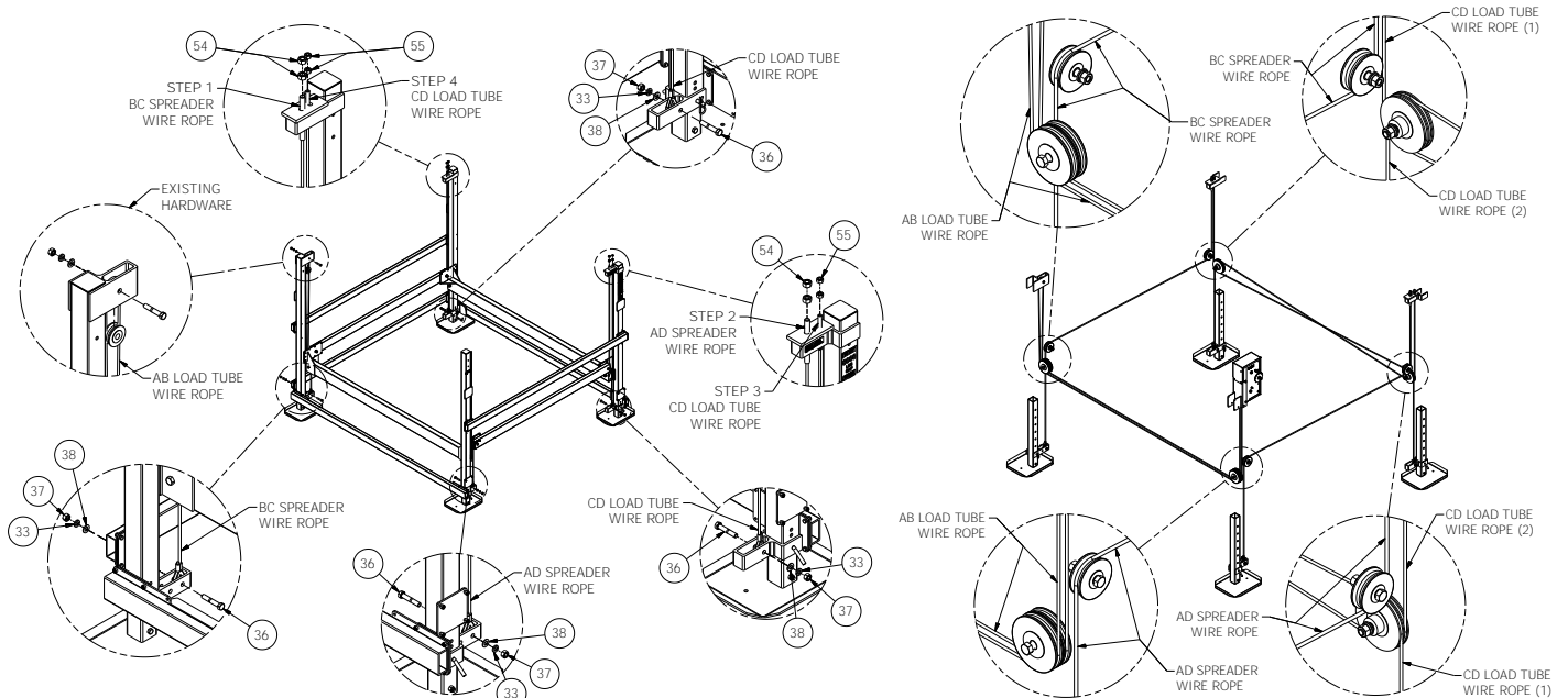
Cable Reeving & Adjustment
