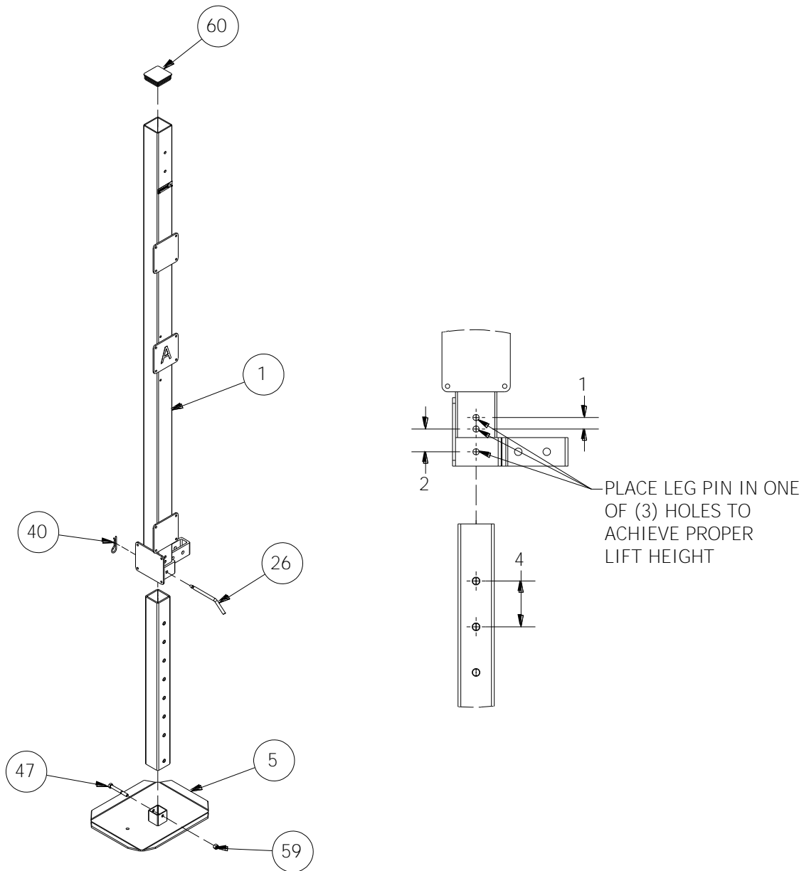
Vertical Leg Assembly
