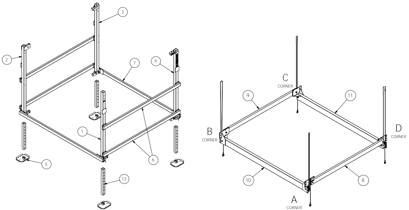
Vertical Lift Frame & Platform Assembly
