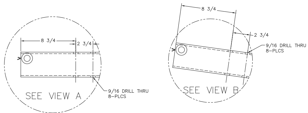
Figure 2-2A. HL4K (48" Lift) Drilling liftarms.
