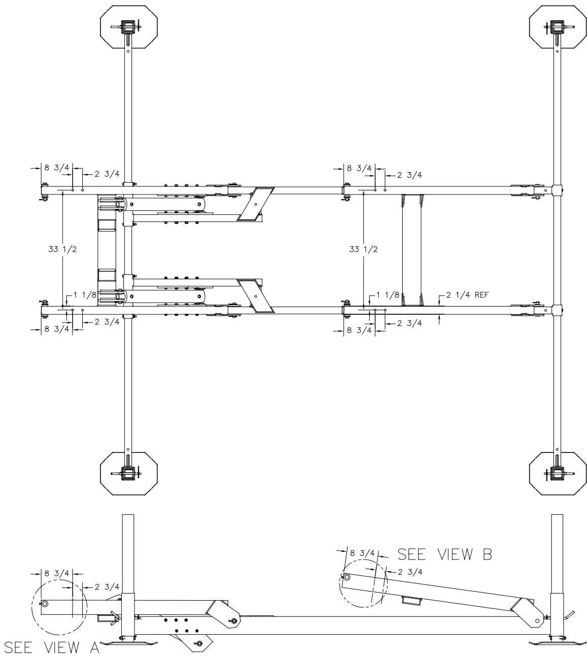
Figure 2-2A. HL4K (48" Lift) Drilling liftarms.
