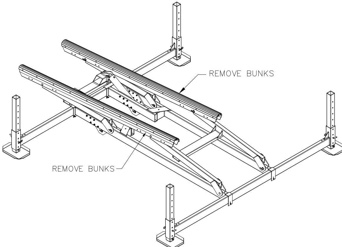
Figure 2-1A. HL4K (48" Lift) Remove Bunks for Drilling liftarms.
