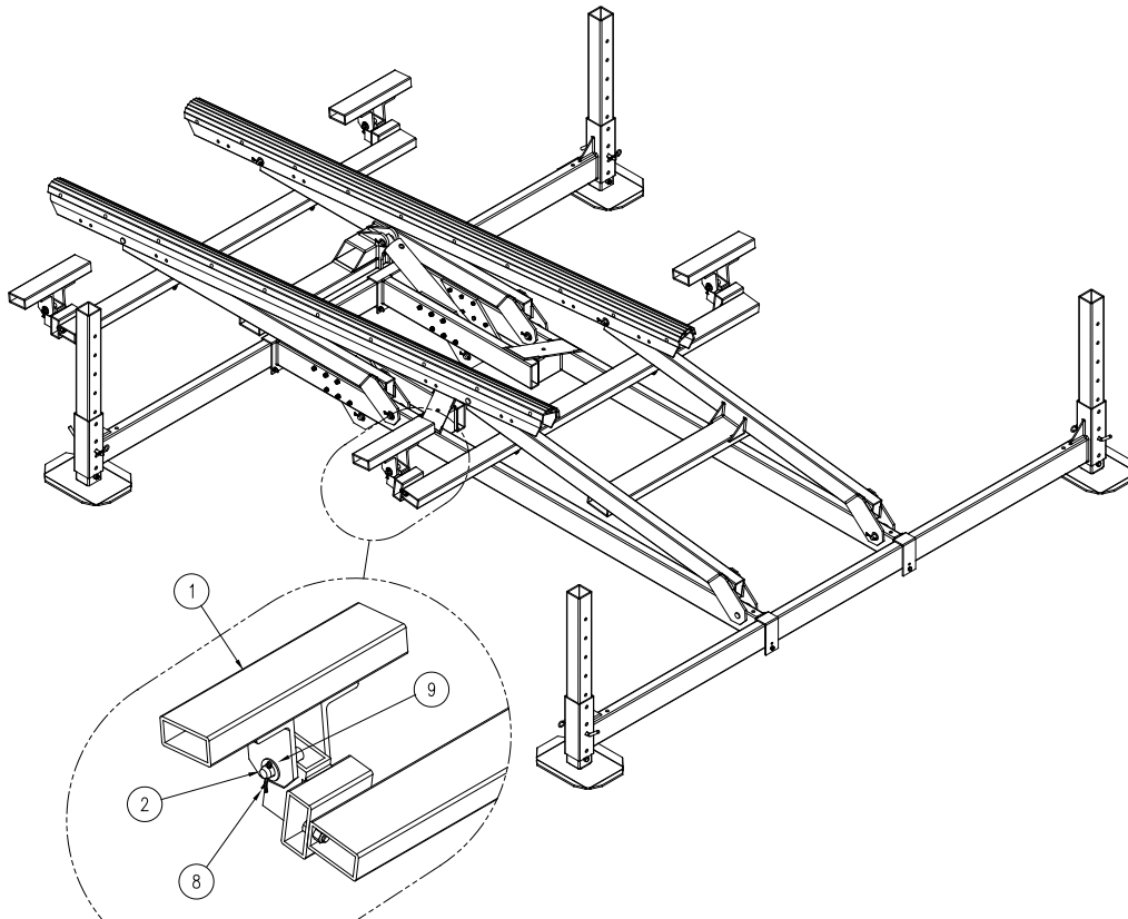
Figure 2-5B. HL4K (60" Lift) Pontoon Bunk Support Weldment
