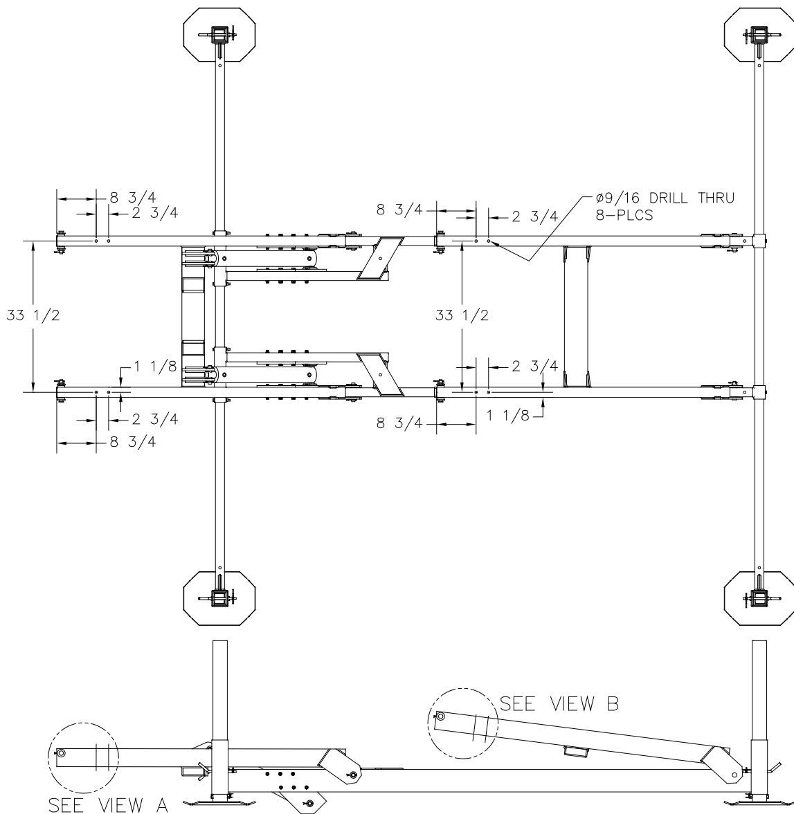
Figure 2-2B. HL4K (60" Lift) Drilling liftarms.
