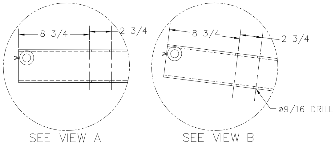
Figure 2-3B. HL-4K (60" Lift) Drilling liftarms
